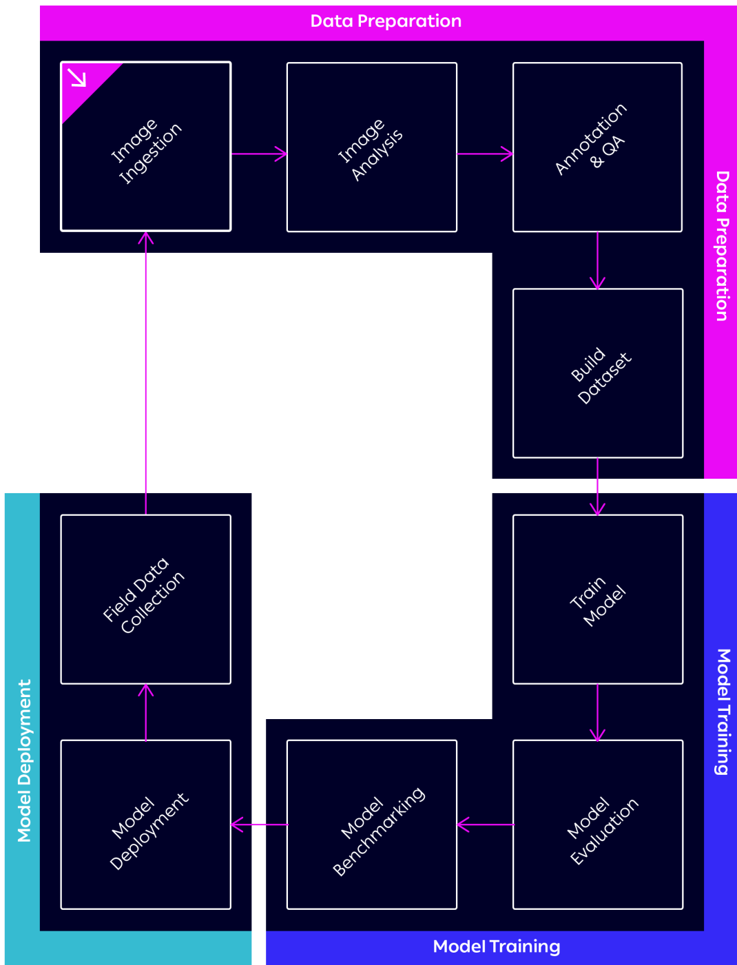
Diagram of Neural Guard's automated pipeline
